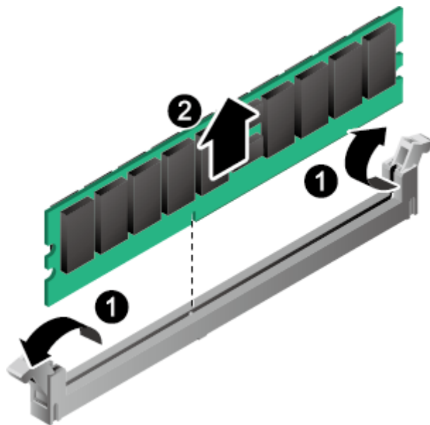
图6-71 拆卸 DIMM
