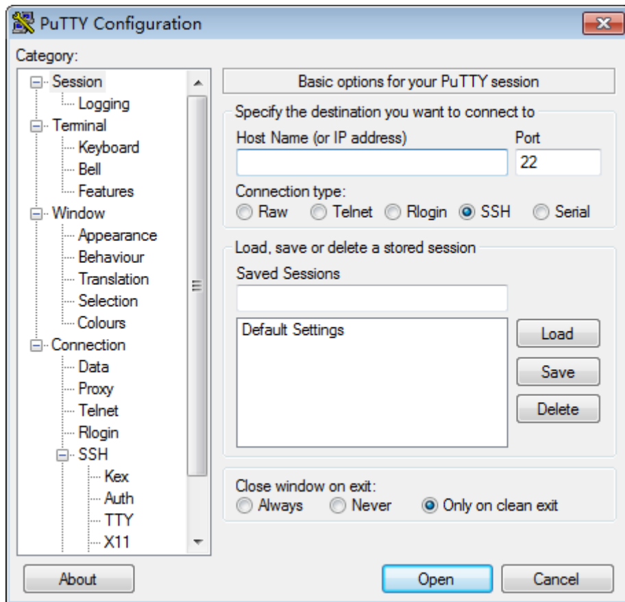
图8-23 PuTTY Configuration
