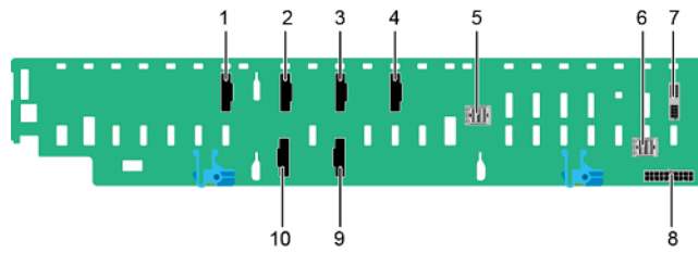
图3-22 8x2.5 SAS/SATA+12x2.5 NVMe 硬盘背板
